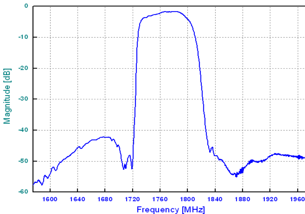
Frequency Response
